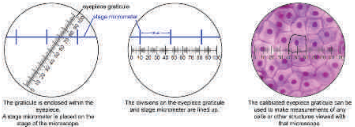
Figure 1.49: Calibrating, then using an eyepiece graticule.
